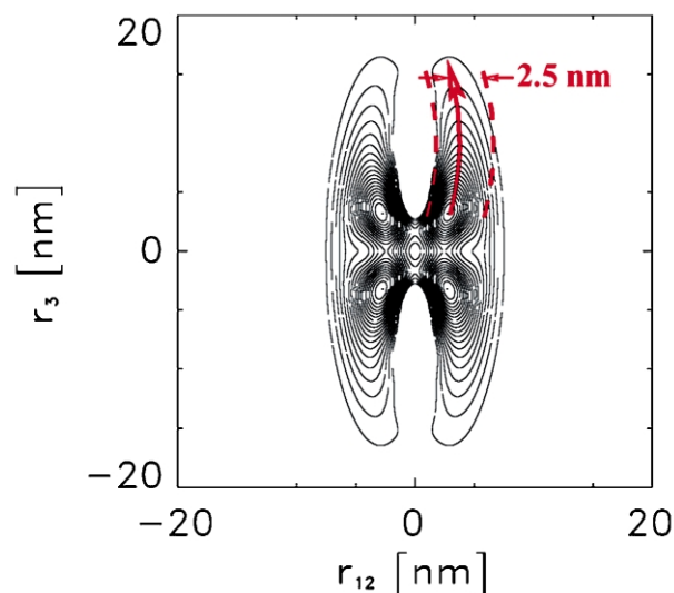
Fig. 13. Ultimate nanostructure of the polymer matrix of Nafion ® 117. Positive contours of the domain peaks from the CDF. Strained state at \varepsilon = 1.25 . The arrow indicates the correlation between domain height and orientation, starting from short and poorly parallelized domains. Broken lines indicate the estimation of the almost constant domain diameters.
