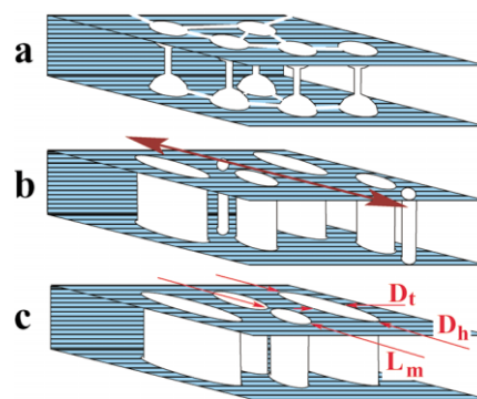
Fig. 8. Sketch of a void-layer structure and its evolution during straining of Nafion 117 ® that is compatible with the nanostructure data extracted from the measured MAXS patterns. (a) native material. (b) medium elongation. The straining direction is indicated by a double arrow. (c) high elongation. The domain thickness, D_t , domain height, D_h , and the meridional long period of the CDF, L_m , that is resulting from struts crossing the void-layers.
