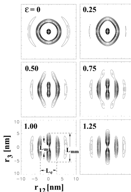
Fig. 6. Strained Nafion 117 ® . Contours of the negative peaks (related to the long periods) in the CDF of the MAXS structure. Straining direction ( r_3 ) is vertical. L_m : Most probable long period in meridional direction. L_{mm} : Maximum long period in meridional direction. L_e : Average long period in equatorial direction.
