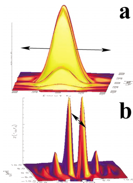
Fig. 5. Nafion 117 ® at \varepsilon = 1.25 . Domain dimension peaks from the CDF z(r_{12}, r_3) viewed (a) perpendicular and (b) parallel to the straining direction, r_3 , indicated by double head arrows.
