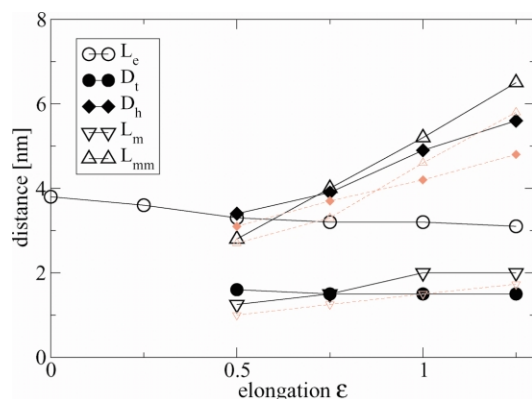
Fig. 7. MAXS-related nanostructure of Nafion 117 ® in strained and relaxed state. Evaluation of the CDFs results in dimensions of the domains and the long periods as a function of elongation. Solid lines and large symbols: sample strained. Dashed lines and small symbols: sample after relaxation from strain. In equatorial direction changes upon strain are small and not shown here. L_e : long period in equatorial direction. D_t : domain thickness (equatorial direction). D_h : domain height. L_m : meridional long period, most probable value in straining direction. L_{mm} : meridional long period, maximum value.
