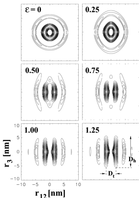
Fig. 4. Strained Nafion ® 117. Contours of the positive peaks (related to the domains) in the CDF z_M(r_{12}, r_3) of the MAXS structure. Straining direction ( r_3 ) is vertical. D_t : Average domain thickness. D_h : Maximum domain height
