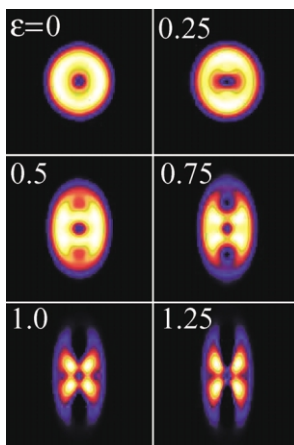
Fig. 9. Nanostructure of the polymer matrix of Nafion® 117 during elongation (transverse to MD). CDFs z(r_{12}, r_3) , -20 \text{ nm} \leq r_{12}, r_3 \leq 20 \text{ nm} , (domain peaks) as a function of elongation \varepsilon .
