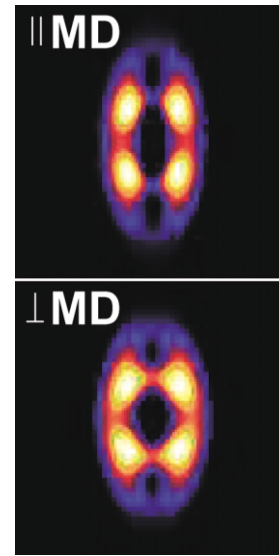
Fig. 10. Different straining directions and the nanostructure of Nafion 117. The CDF domain peaks are shown at \varepsilon = 1.0 . Straining direction is vertical. Narrow peaks (top) when straining in MD. Broader domain peaks (bottom) when straining in TD. Peak positions are identical.
