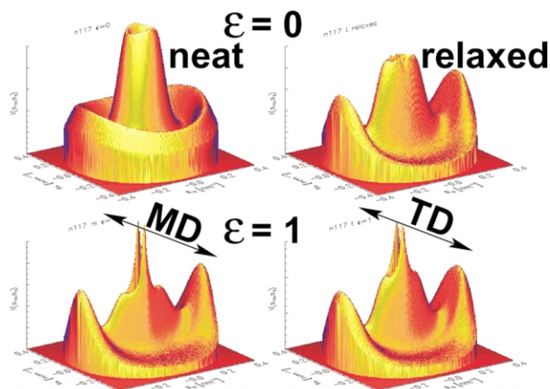
Fig. 1. Dry Nafion® 117 film. SAXS intensity I(s_{12}, s_3) , (-0.4 \text{ nm}^{-1} \leq s_{12}, s_3 \leq 0.4 \text{ nm}^{-1} ; long sample-to-detector distance) before, during and after straining to \varepsilon = 1 . Bottom left: Strained in machine direction (MD). Bottom right: strained in transverse direction (TD).
