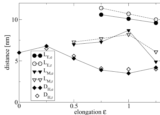
Fig. 11. Comparing strained and relaxed state of the nanostructure of the polymer matrix of Nafion 117 as a function of elongation. Domain dimensions and long periods as evaluated from the CDFs. Filled symbols: sample strained. Open symbols: sample after relaxation from strain. L_E : long period in equatorial direction (observed only at high elongation). L_M : meridional long period (maximum of narrow peak). D_H : most probable domain heights (in oblique direction).
