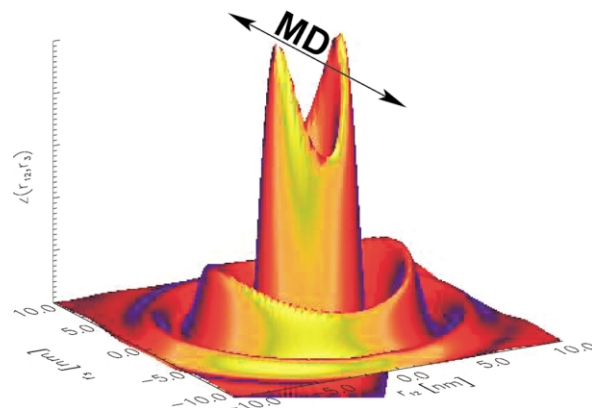
Fig. 3. Multidimensional chord distribution function (CDF) z_M(r_{12}, r_3) of the MAXS structure, (-10 \text{ nm} \leq r_{12}, r_3 \leq 10 \text{ nm}) of Nafion 117® as extruded (domain peaks). Machine direction( MD, r_3 ) is indicated by an arrow.
