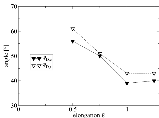
Fig. 12. Domain orientation of the matrix-related nanostructure of Nafion ® 117 in strained (filled symbols) and relaxed state (open symbols) as evaluated from the CDFs. \phi_D is the most probable angle enclosed by the straining direction and the axis of the cylindrical domains.
