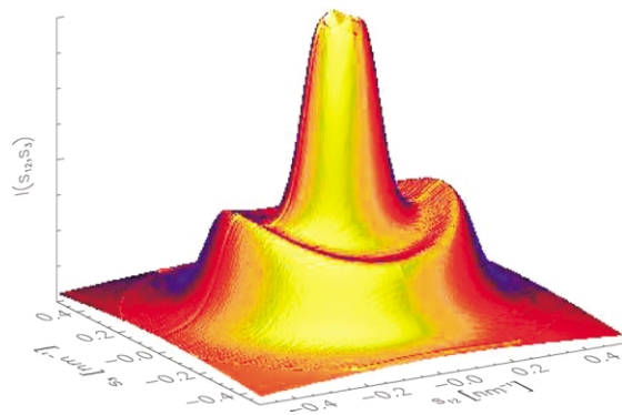
Fig. 2. Neat Nafion® 117. Scattering intensity \{I\}_2(s_{12}, s_3) projected onto the representative plane with the fiber axis chosen in MD. Visible range: -0.5 \text{ nm}^{-1} \leq s_{12}, s_3 \leq 0.5 \text{ nm}^{-1} .
